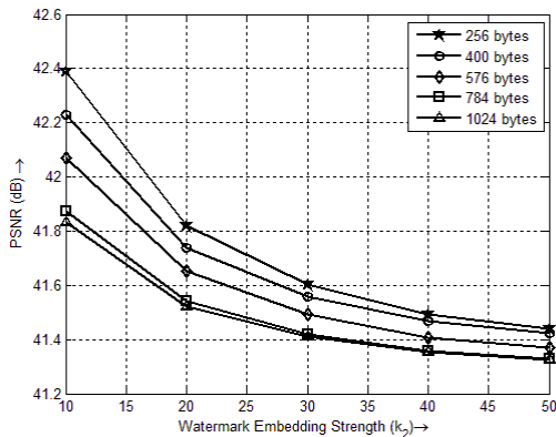
Fig. 6. Curve of Peak Signal to Noise Ratio (PSNR) in dB against Embedding Strength ( k_2 ) for Different Watermark Images having Different Size and Payloads.
