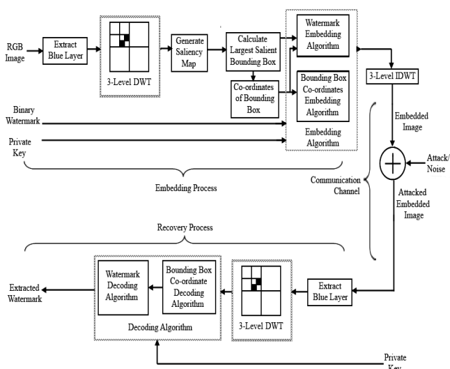
Fig. 1. Block Diagram of Watermark Embedding and Extraction
