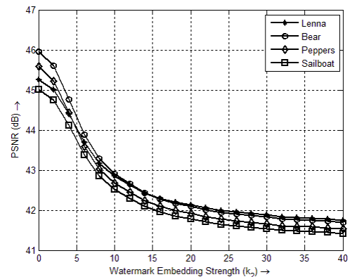
Fig. 5. Curve of Peak Signal to Noise Ratio (PSNR) in dB against Varying Embedding Strength ( k_2 ) for Different Cover Images.
