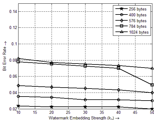
Figure 7. Curve of Bit Error Rate (BER) against Embedding Strength ( k_2 ) for Different Watermark Images Having Different Size and Payloads.
