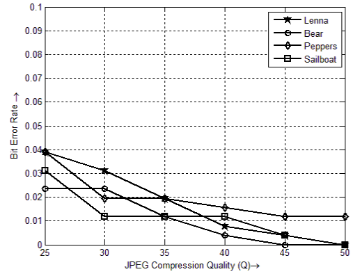
Fig. 4. Curve of Bit Error Rate (BER) against Varying Quality Factor of JPEG Compression ( Q ) for Different Cover Images.
