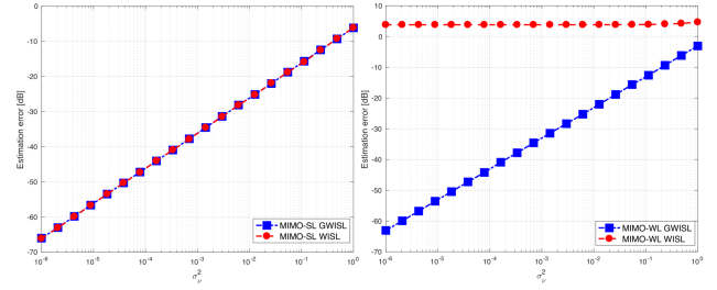
Fig. 2. Estimation error of a 2 \times 2 MIMO-SL (left) and MIMO-WL (right) system for different noise variances.
