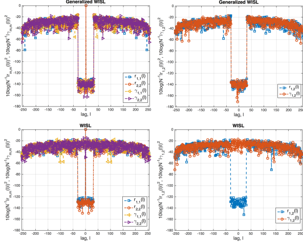
Fig. 1. Correlation and complementary correlation of \{x_m(n)\} using GWISL (top) and WISL (bottom) criterion.
